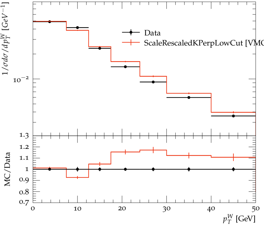
CMS, 8 TeV, W boson pT distribution in muon channel
