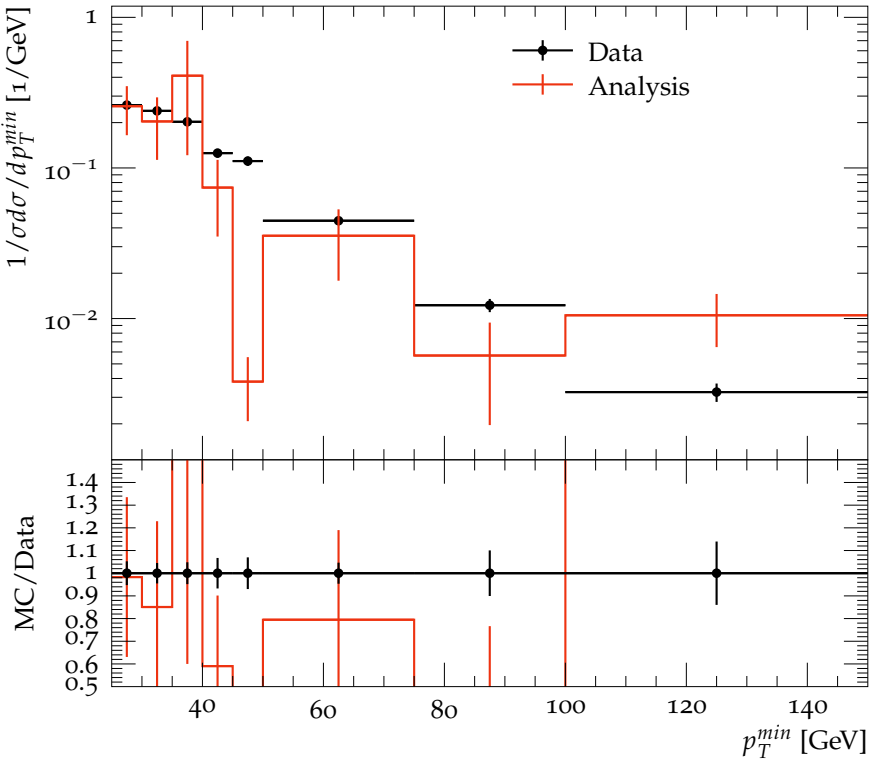
CMS, 13 TeV, W^+W^- , Figure 6 lower left
