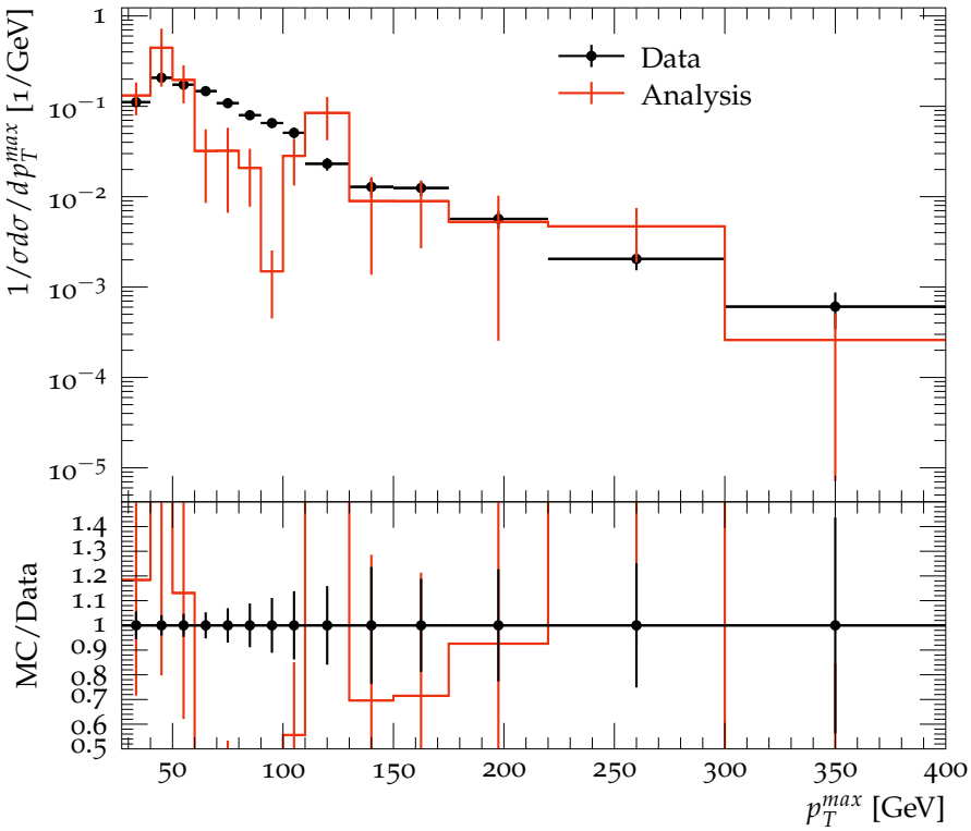
CMS, 13 TeV, W^+W^- , Figure 6 upper right
