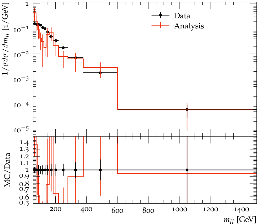
CMS, 13 TeV, W^+W^- , Figure 6 upper left
