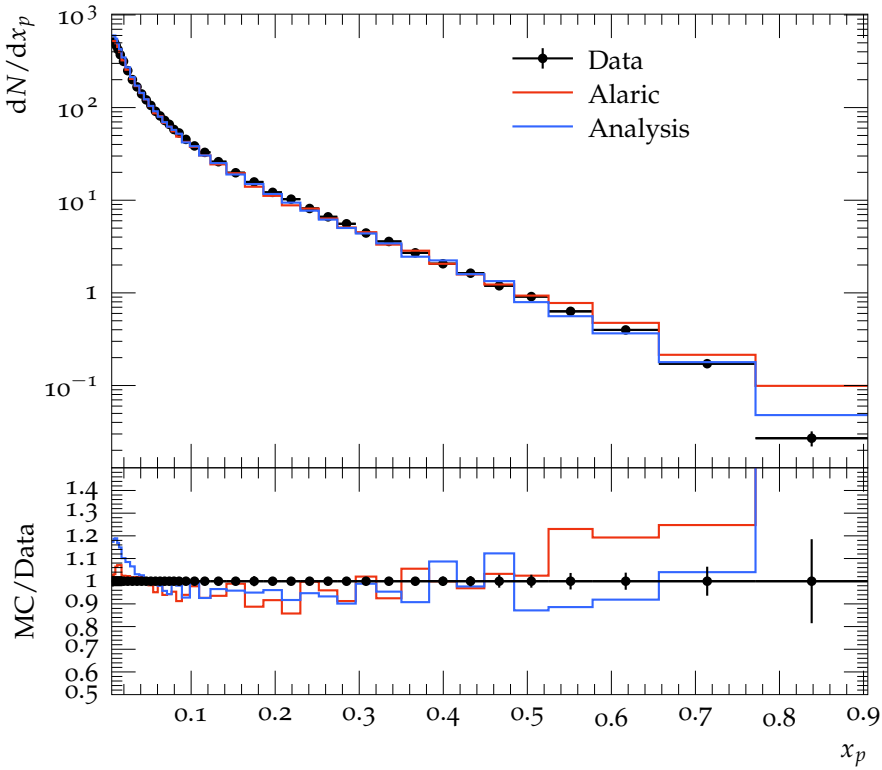
Charged particle scaled Momentum, ( uds ) events
