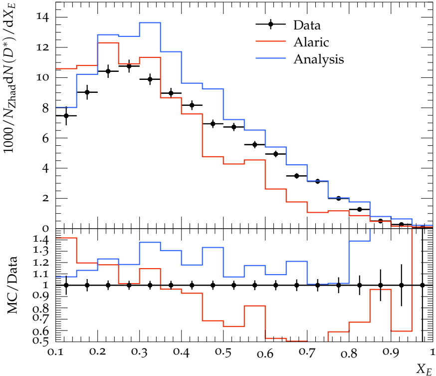
Scaled energy of D^{*\pm} in e^+e^- \rightarrow Z \rightarrow \text{hadronic} at \sqrt{s} = 91.2 \text{ GeV}
