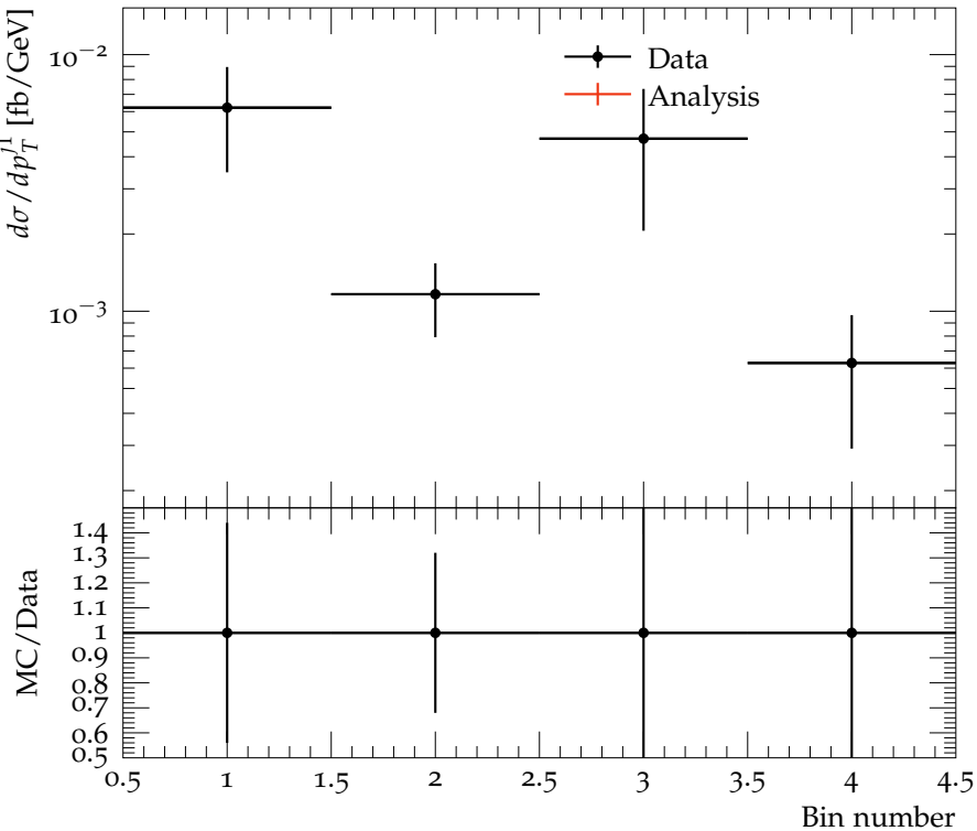
1D differential xsection vs p_T^{j1} in bins of \Delta\phi_{jj} in VBF region
