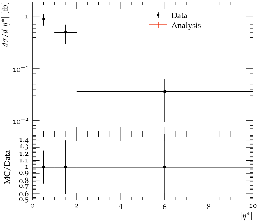
1D differential xsection vs |\eta^*| in VBF region
