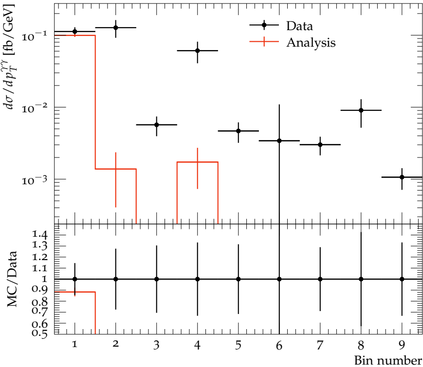
1D differential xsection vs p_T^{\gamma\gamma} in bins of \tau_{C,j1}
