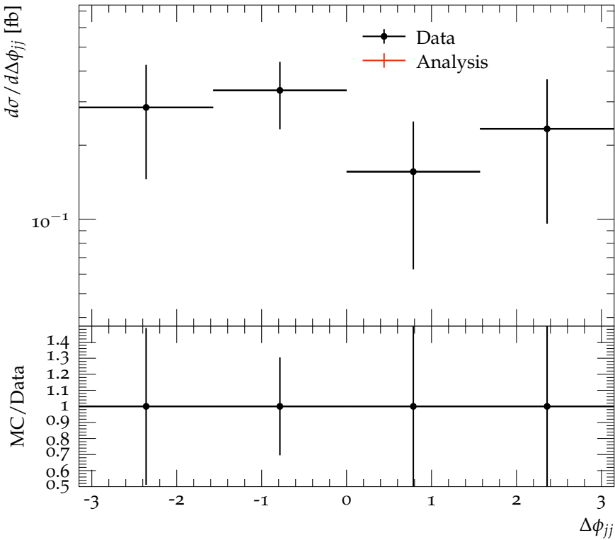
1D differential xsection vs \Delta\phi_{jj} in VBF region
