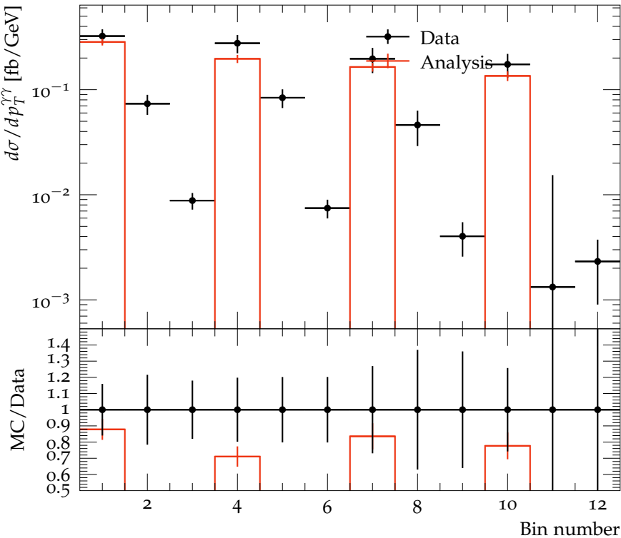
1D differential xsection vs p_T^{\gamma\gamma} in bins of |y_{\gamma\gamma}|
