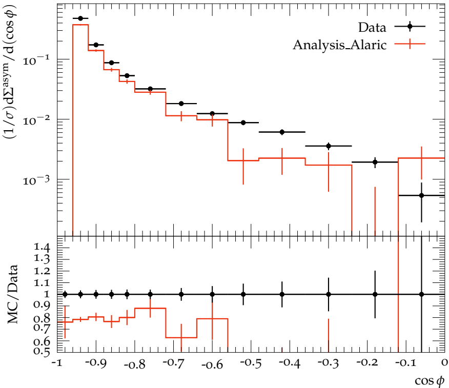
Transverse EEC asymmetry for 1100 \text{ GeV} < H_{T2} < 1400 \text{ GeV}
