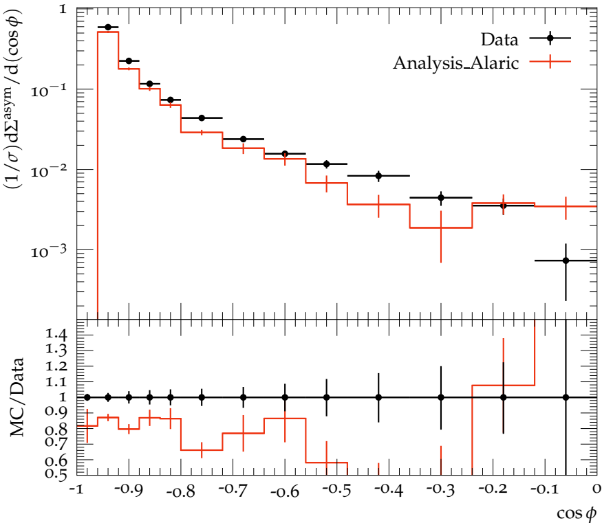
Transverse EEC asymmetry for 900 \text{ GeV} < H_{T2} < 1000 \text{ GeV}
