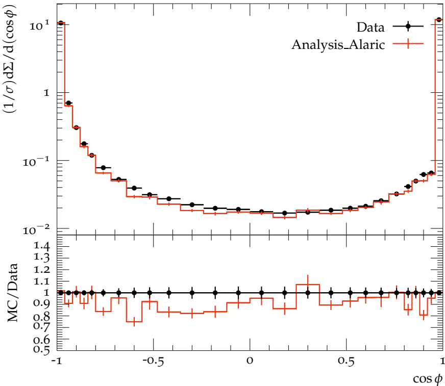
Transverse EEC for 850 \text{ GeV} < H_{T2} < 900 \text{ GeV}
