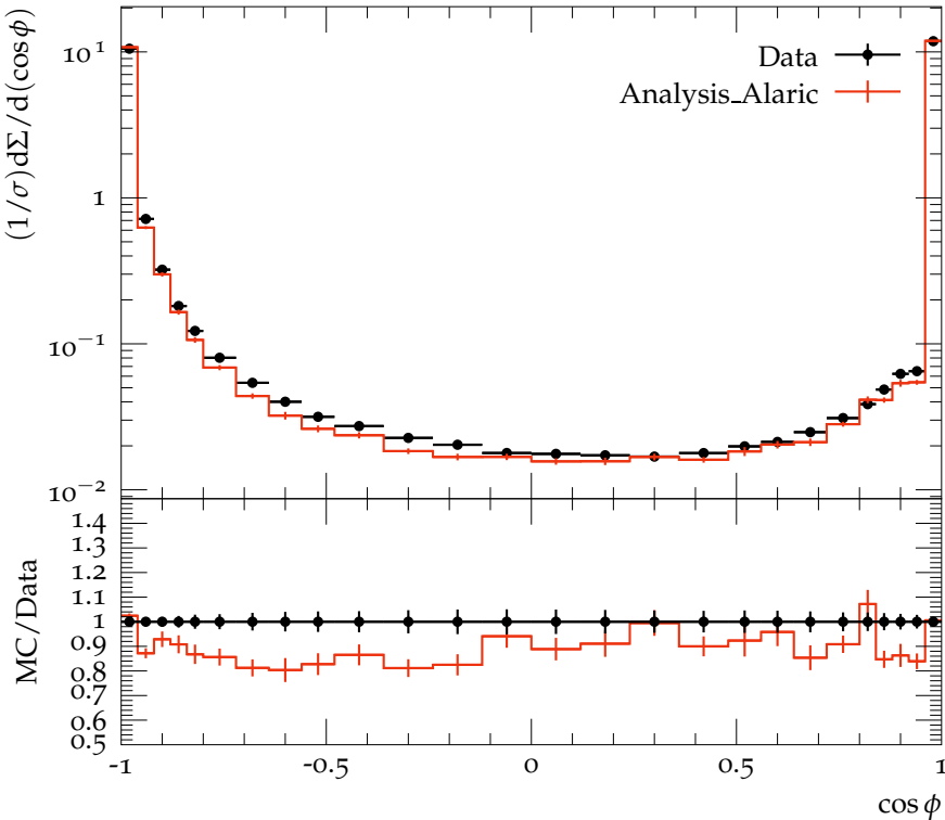
Transverse EEC for 800 \text{ GeV} < H_{T2} < 850 \text{ GeV}
