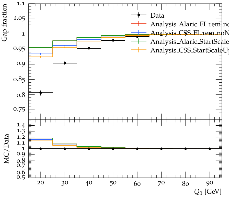
Gap fraction as a function of Q_0 for events satisfying 1 < \Delta y \leq 2
