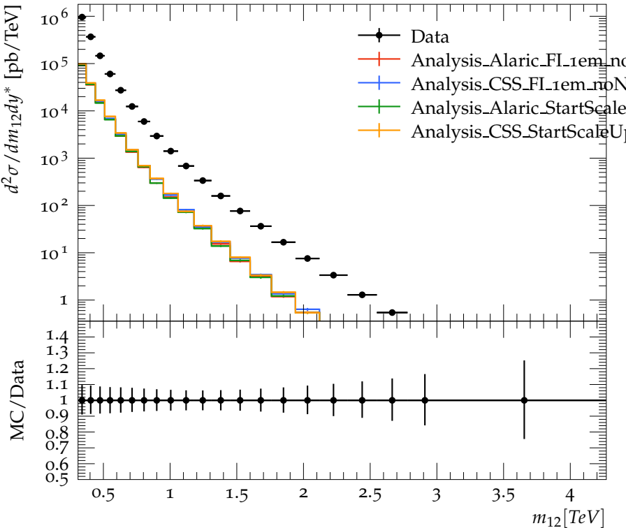
Dijet double-differential cross sections ( 0.5 < y^* < 1.0 ), R=0.6
