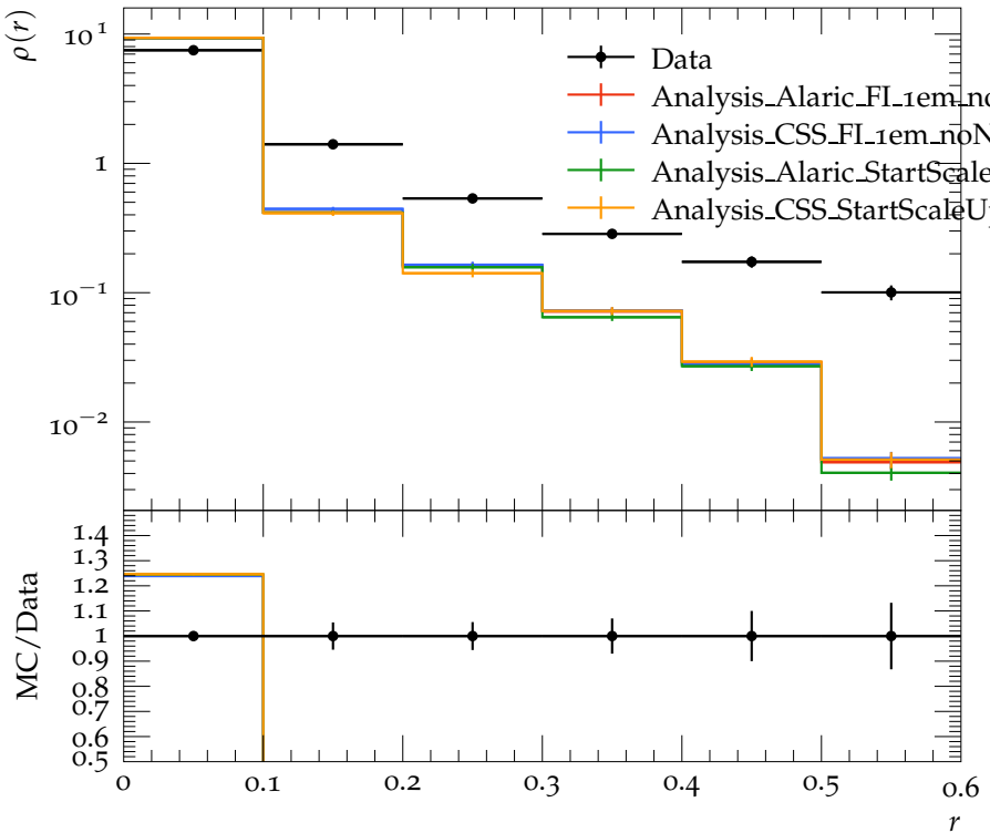
Jet shape \rho for p_{\perp} \in 310\text{--}400 GeV, y \in 0.0\text{--}2.8
