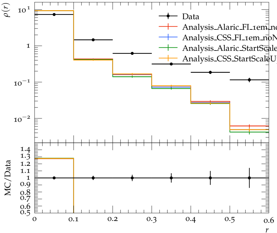
Jet shape \rho for p_{\perp} \in 260\text{--}310 GeV, y \in 0.0\text{--}2.8
