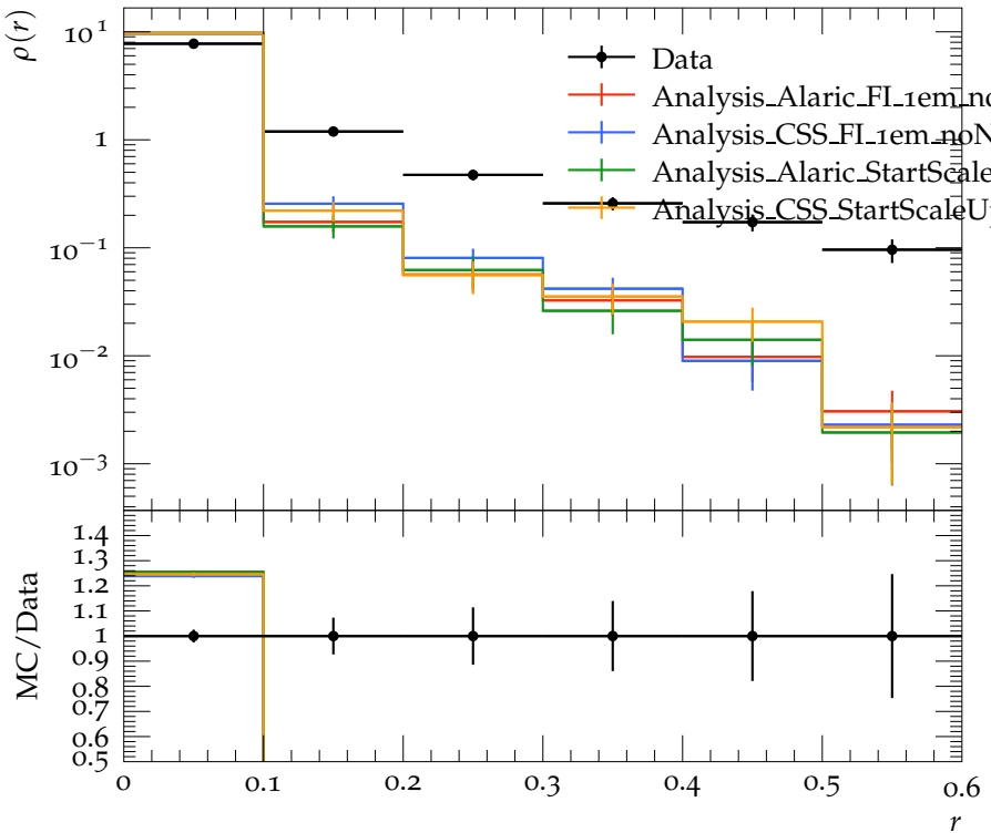
Jet shape \rho for p_{\perp} \in 260\text{--}310 GeV, y \in 2.1\text{--}2.8
