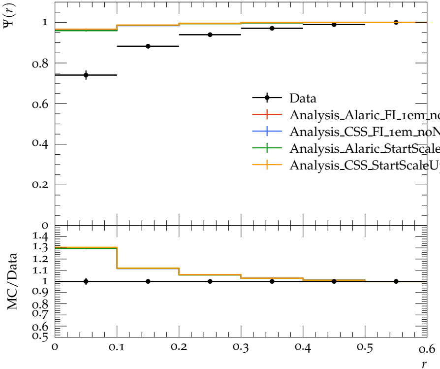
Jet shape \Psi for p_{\perp} \in 210\text{--}260 GeV, y \in 2.1\text{--}2.8
