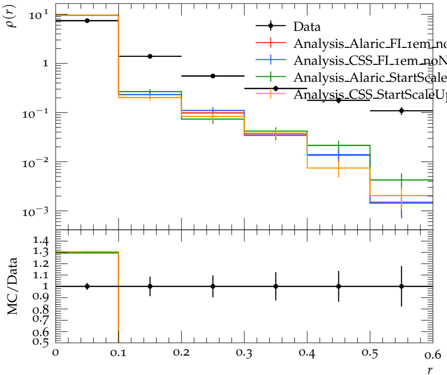
Jet shape \rho for p_{\perp} \in 210\text{--}260 GeV, y \in 2.1\text{--}2.8
