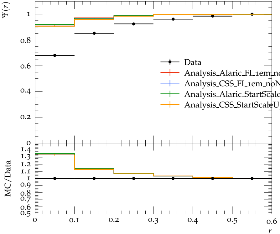
Jet shape \Psi for p_{\perp} \in 210\text{--}260\text{ GeV} , y \in 0.0\text{--}0.3
