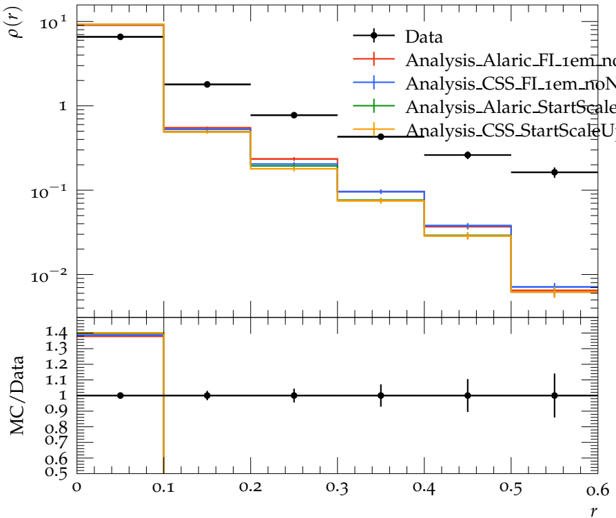
Jet shape \rho for p_{\perp} \in 160\text{--}210 GeV, y \in 0.3\text{--}0.8
