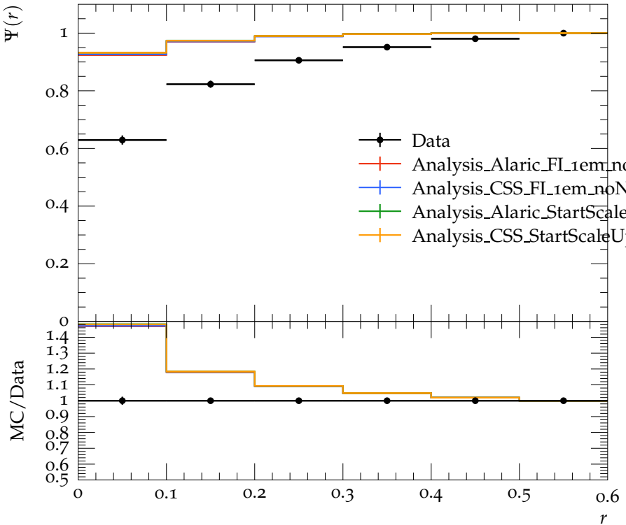
Jet shape \Psi for p_{\perp} \in 110\text{--}160\text{ GeV} , y \in 0.0\text{--}2.8
