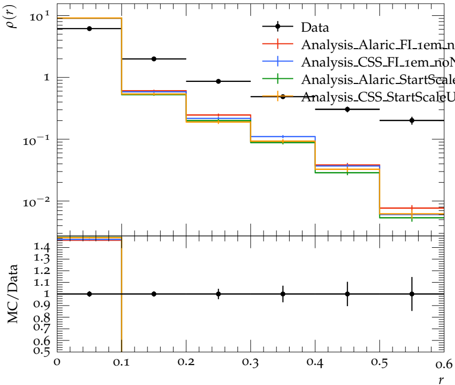
Jet shape \rho for p_{\perp} \in 110\text{--}160 GeV, y \in 0.0\text{--}0.3
