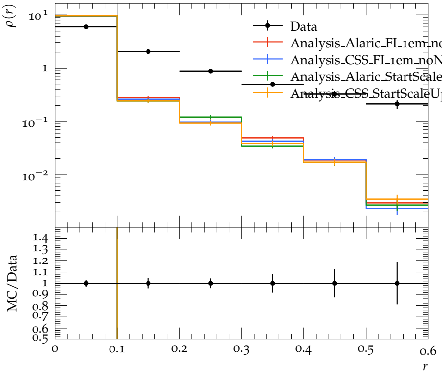
Jet shape \rho for p_{\perp} \in 80\text{--}110\text{ GeV} , y \in 2.1\text{--}2.8
