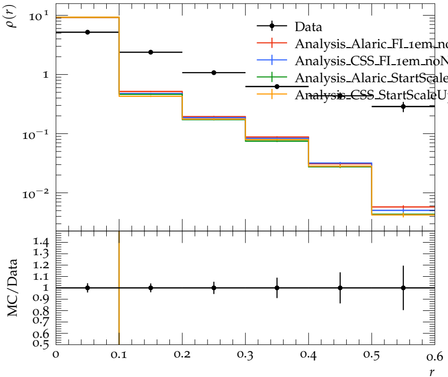
Jet shape \rho for p_{\perp} \in 60\text{--}80\text{ GeV} , y \in 0.0\text{--}2.8
