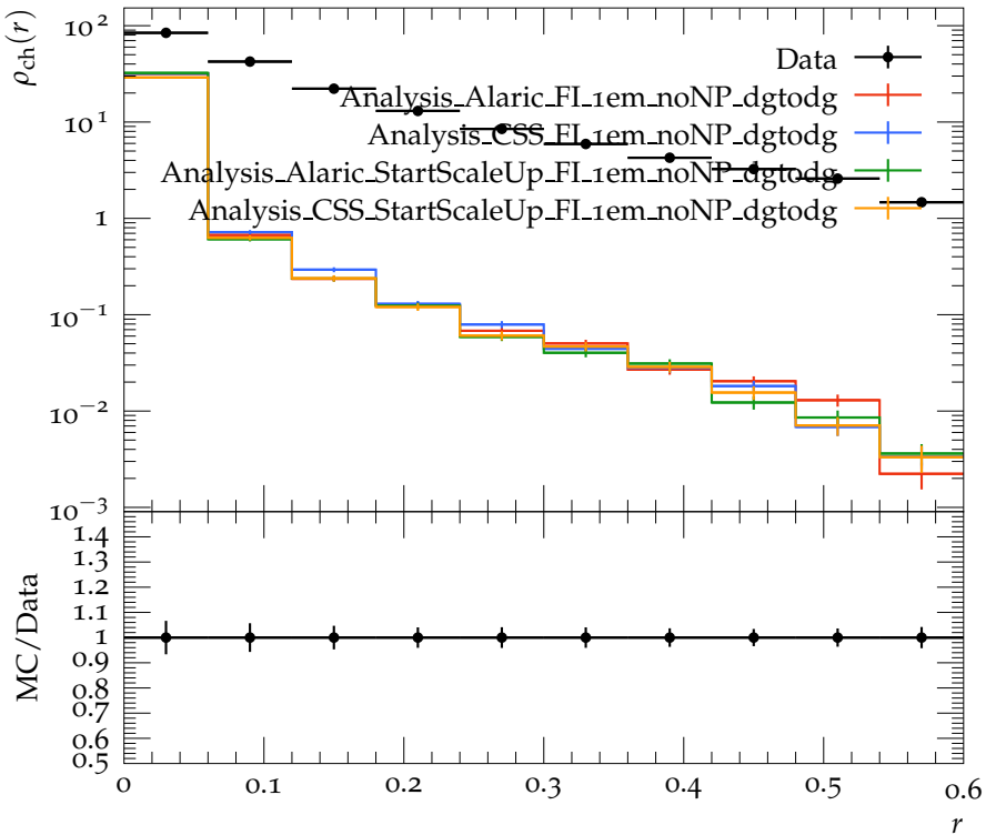
Density of charged particles for 40 \text{ GeV} < p_{T \text{ jet}} < 60 \text{ GeV}
