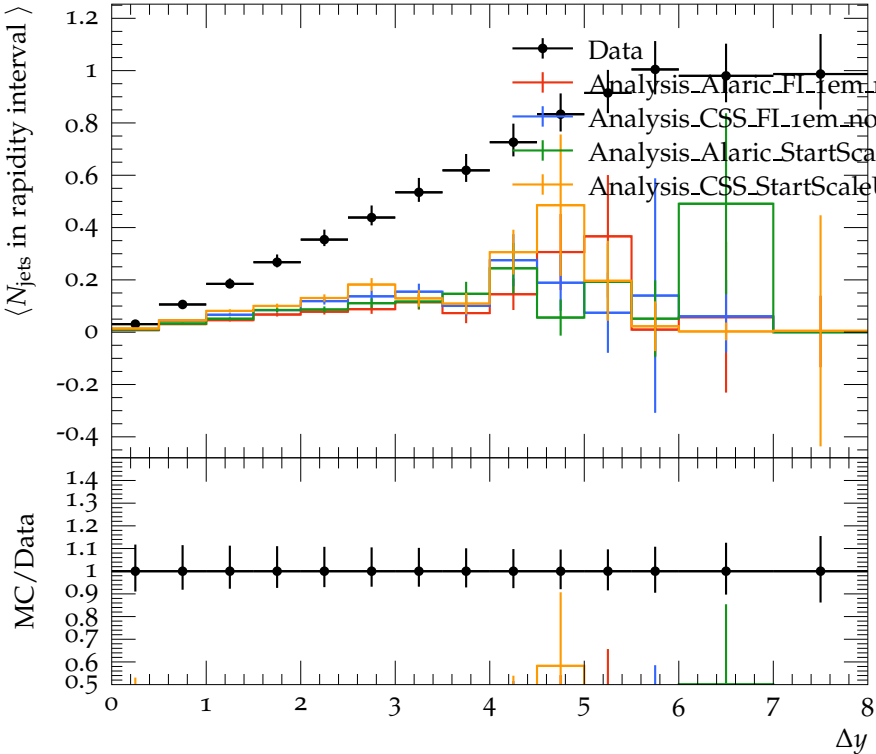
\langle N_{\text{jets in rapidity interval}} \rangle as a function of \Delta y
