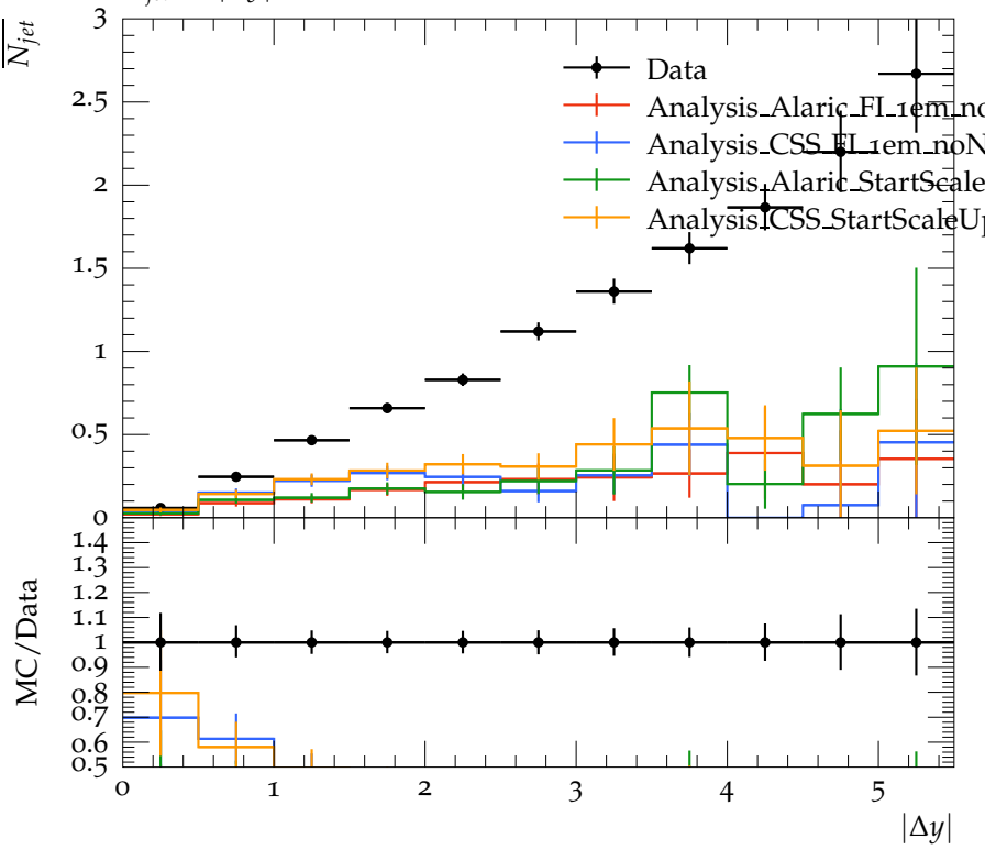
\overline{N}_{jet} vs |\Delta y| for 210 < \overline{P}_T < 240 , Fwd/Bwd
