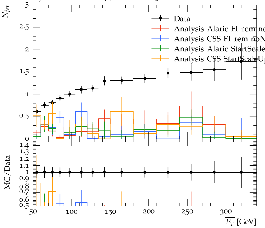
\overline{N}_{jet} vs \overline{P}_T for 4 < |\Delta y| < 5 , Leading Jet
