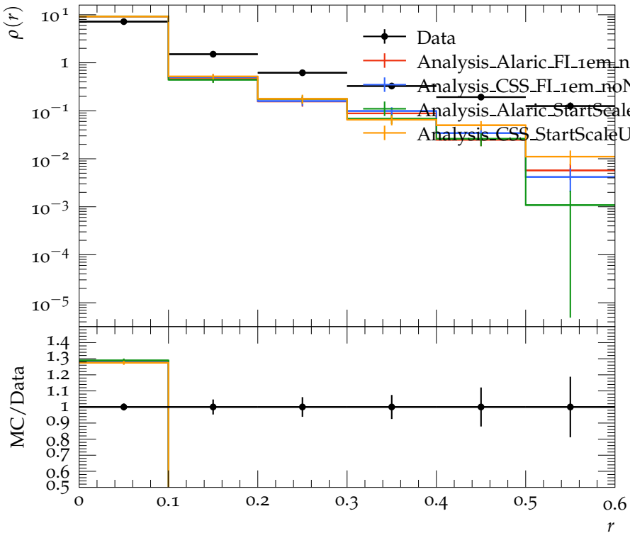
Jet shape \rho for p_{\perp} \in 210\text{--}260 GeV, y \in 1.2\text{--}2.1
