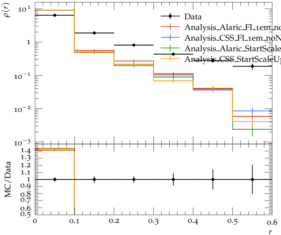
Jet shape \rho for p_{\perp} \in 110\text{--}160\text{ GeV} , y \in 1.2\text{--}2.1
