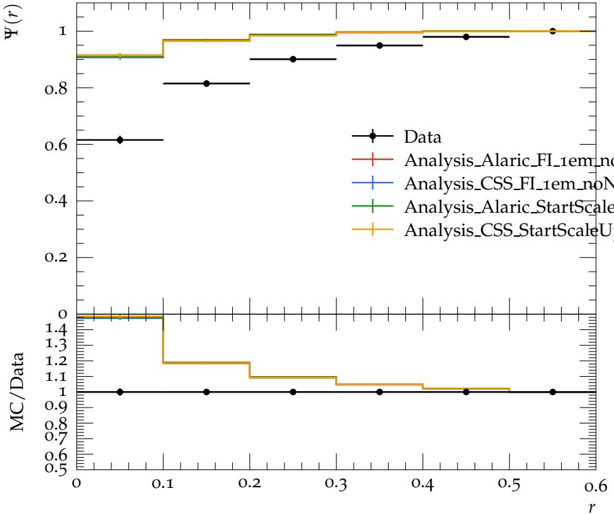
Jet shape \Psi for p_{\perp} \in 110\text{--}160\text{ GeV} , y \in 0.0\text{--}0.3
