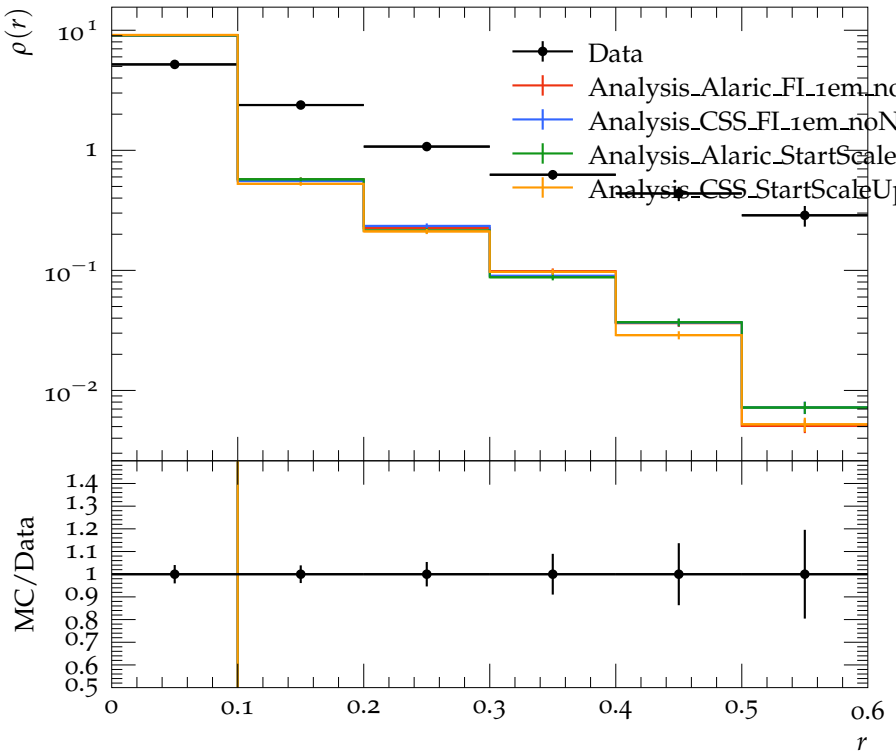
Jet shape \rho for p_{\perp} \in 60\text{--}80\text{ GeV} , y \in 0.0\text{--}2.8
