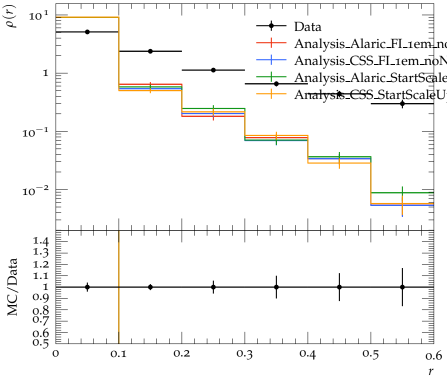
Jet shape \rho for p_{\perp} \in 60\text{--}80\text{ GeV} , y \in 0.0\text{--}0.3
