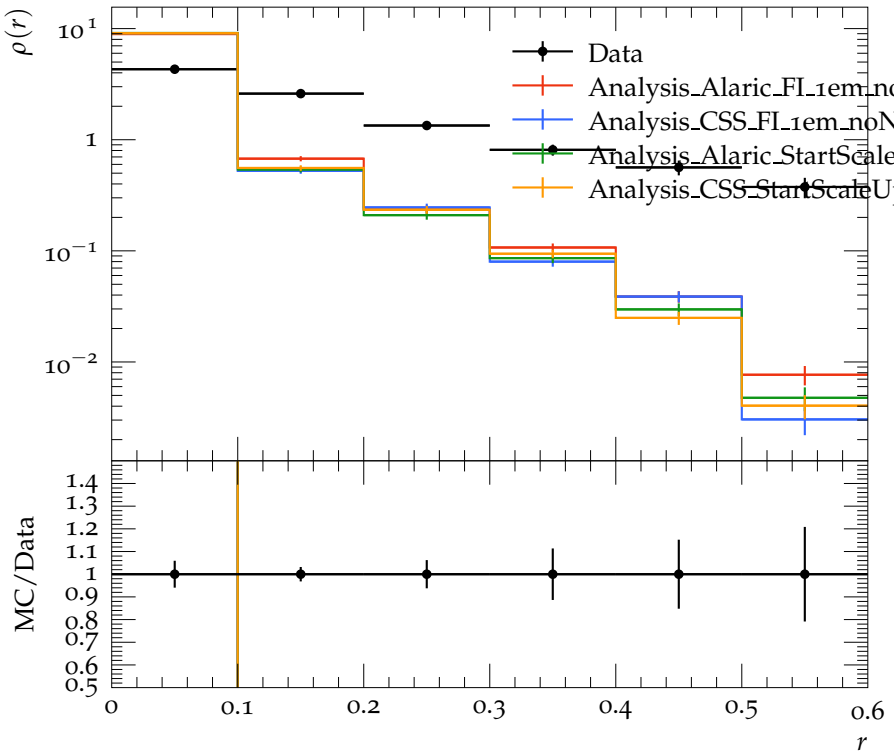
Jet shape \rho for p_{\perp} \in 40\text{--}60 GeV, y \in 0.0\text{--}0.3
