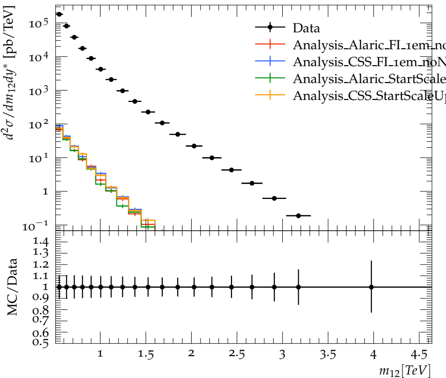
Dijet double-differential cross sections ( 1.0 < y^* < 1.5 ), R=0.6
