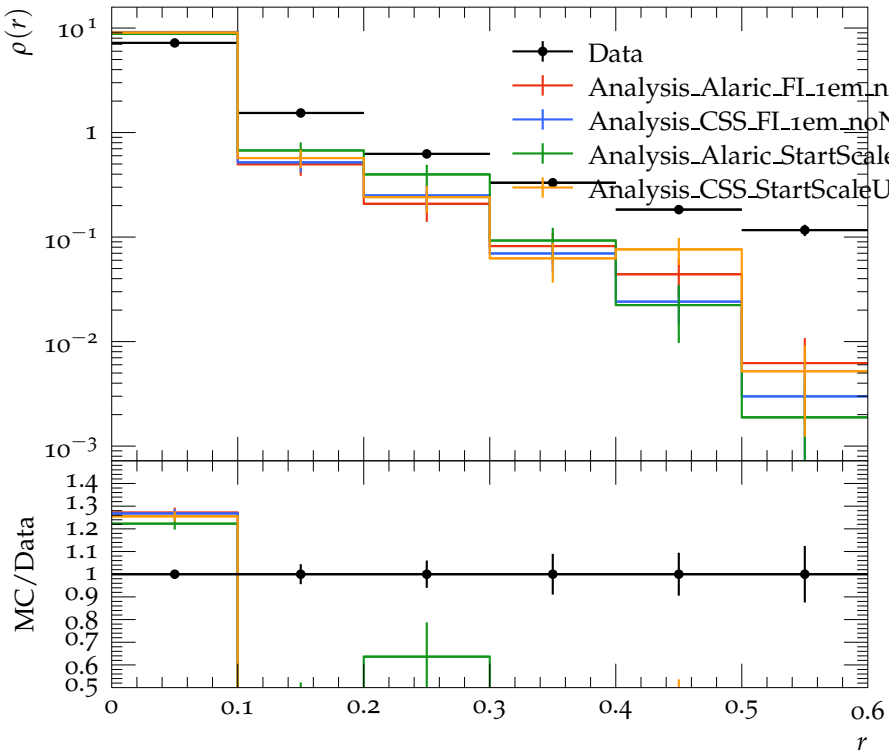
Jet shape \rho for p_{\perp} \in 260\text{--}310 GeV, y \in 0.3\text{--}0.8
