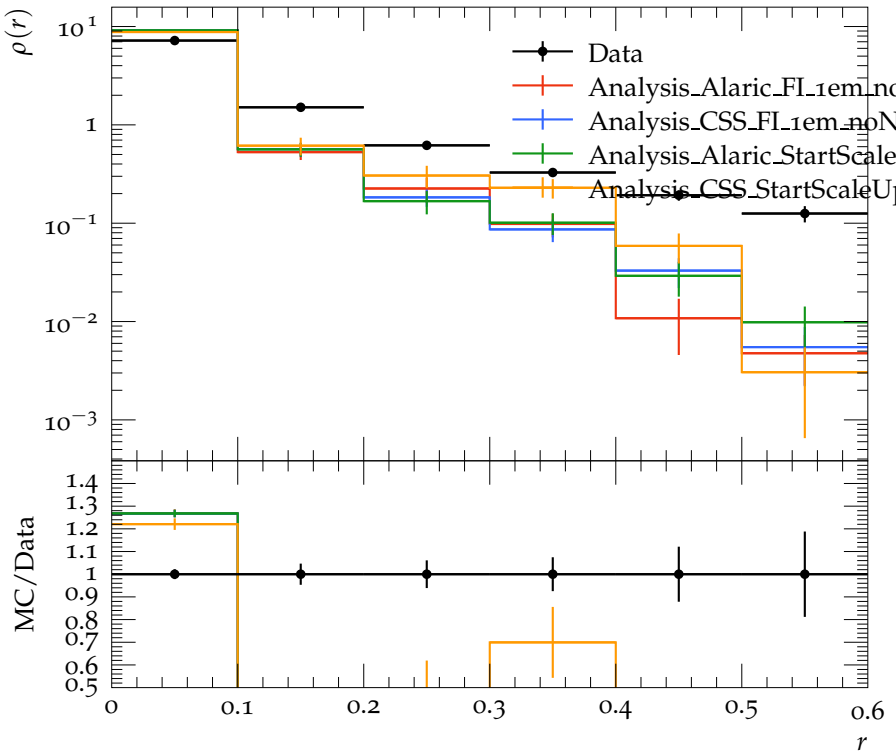
Jet shape \rho for p_{\perp} \in 210\text{--}260 GeV, y \in 1.2\text{--}2.1
