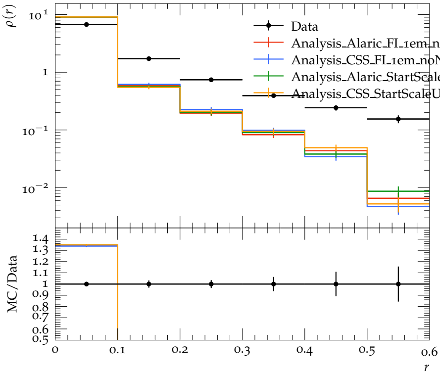
Jet shape \rho for p_{\perp} \in 160\text{--}210 GeV, y \in 0.0\text{--}2.8
