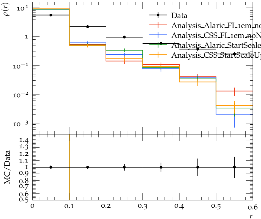
Jet shape \rho for p_{\perp} \in 80\text{--}110\text{ GeV} , y \in 0.0\text{--}0.3
