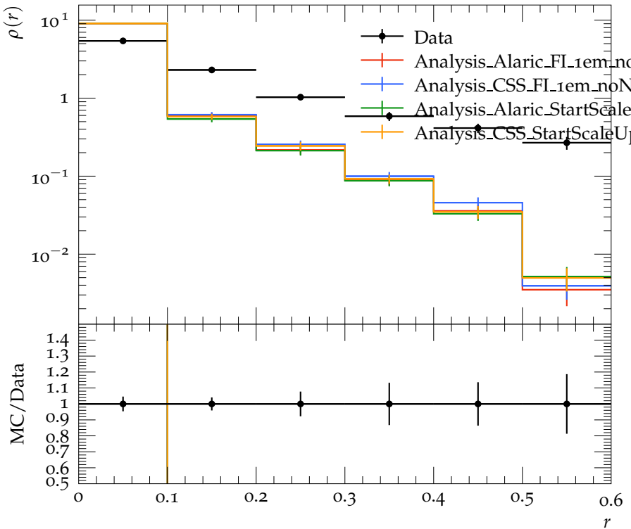
Jet shape \rho for p_{\perp} \in 60\text{--}80\text{ GeV} , y \in 2.1\text{--}2.8
