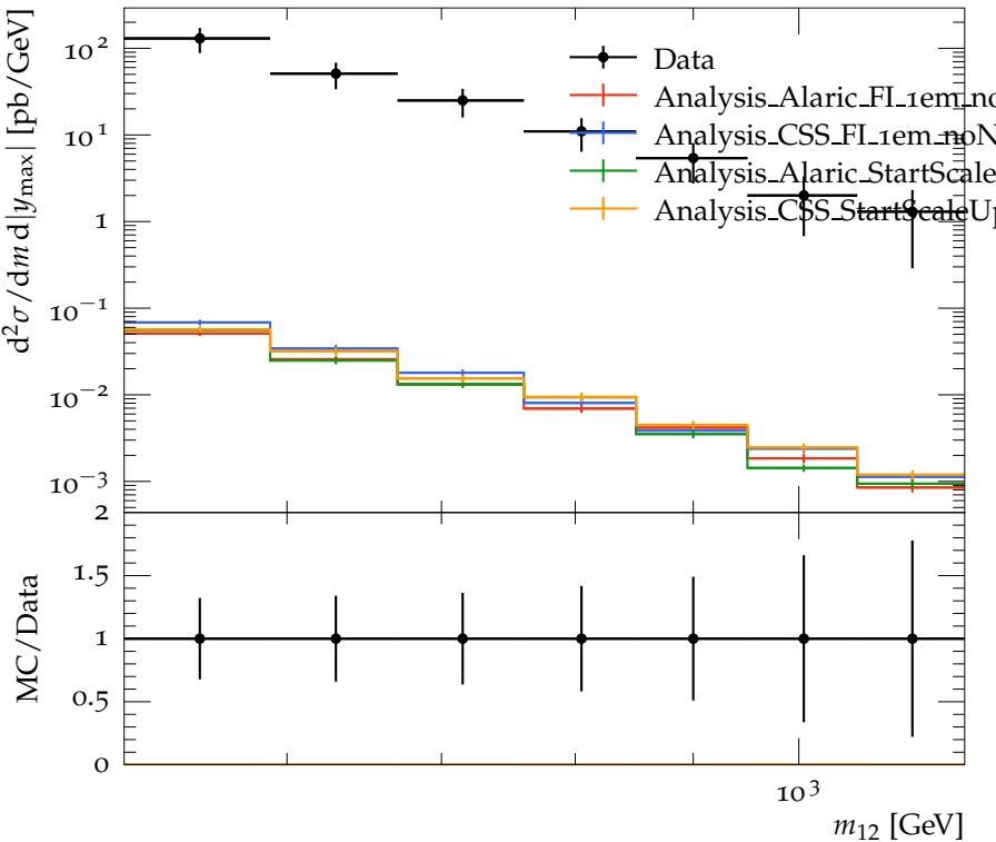
Dijet mass spectrum for 1.2 < |y_{\max}| < 2.1 . anti-KT, R = 0.4 .
