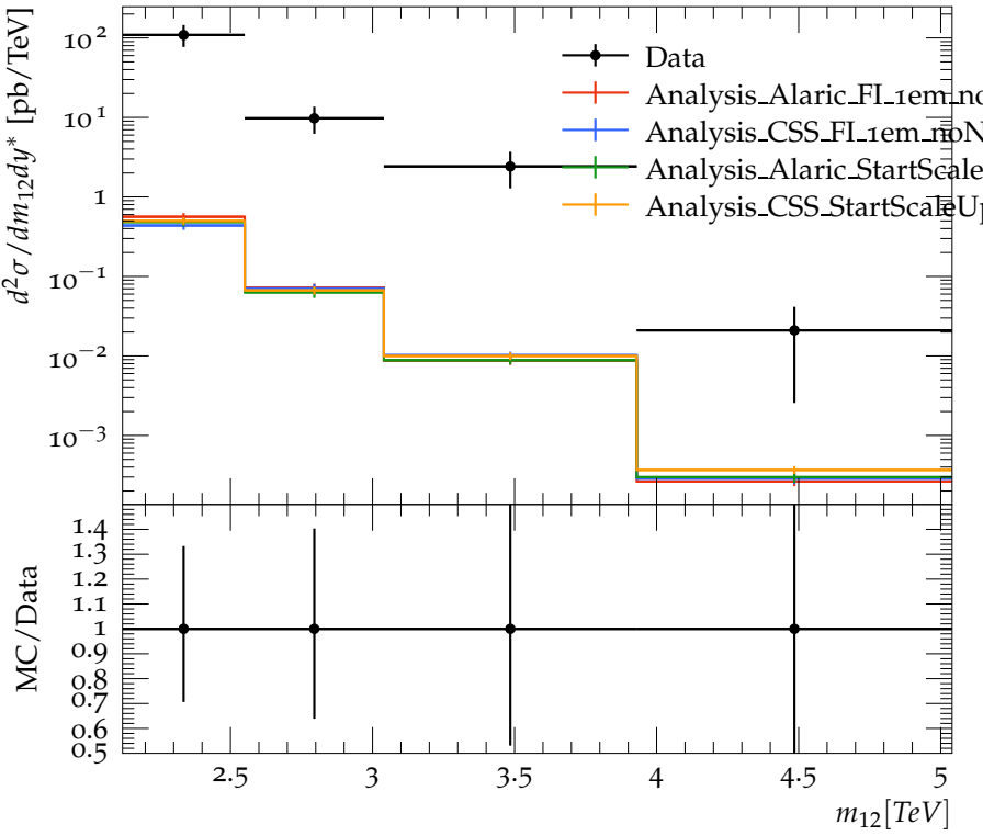
Dijet double-differential cross sections ( 2.5 < y^* < 3.0 ), R=0.6
