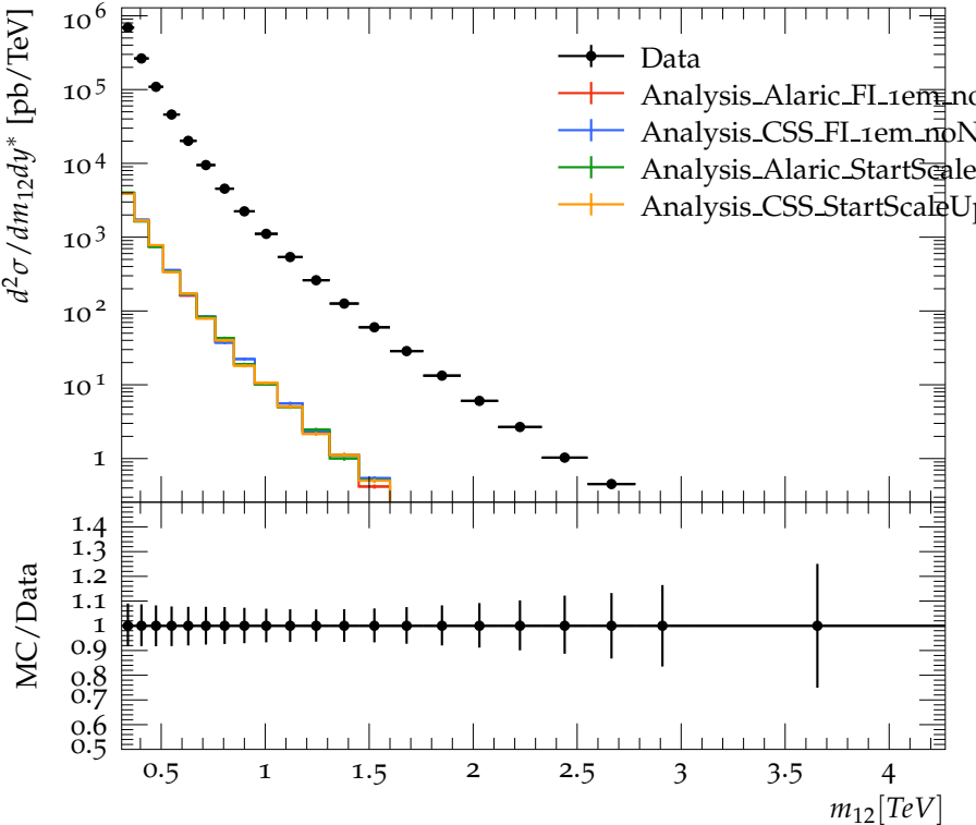
Dijet double-differential cross sections ( 0.5 < y^* < 1.0 ), R=0.4
