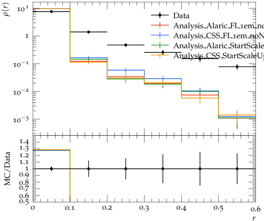
Jet shape \rho for p_{\perp} \in 500\text{--}600 GeV, y \in 0.0\text{--}2.8
