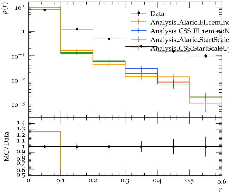
Jet shape \rho for p_{\perp} \in 310\text{--}400 GeV, y \in 1.2\text{--}2.1
