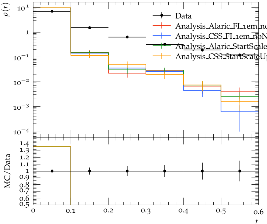
Jet shape \rho for p_{\perp} \in 260\text{--}310 GeV, y \in 0.8\text{--}1.2
